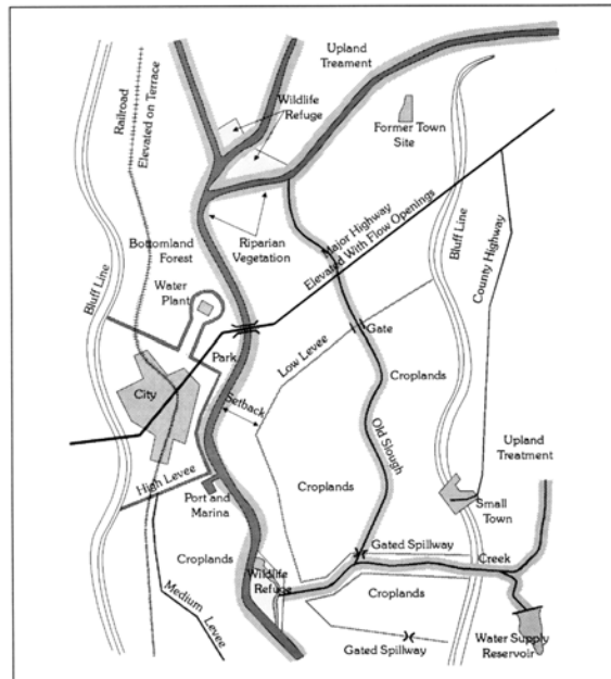
Figure 4.1 A Typical Reach of a 21 st Century Floodplain.
